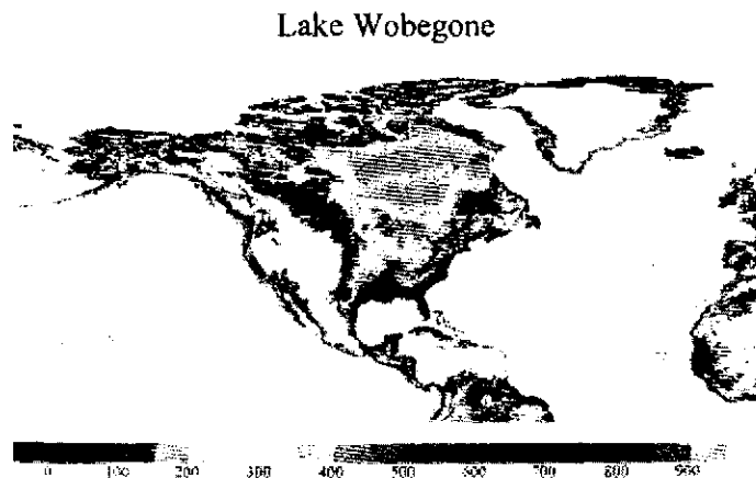
Figure 38. The water contributing one meter of sea level rise could be stored in a lake formed by placing 200 meter high dams at the indicated locations in Canada. This lake would cover a substantial area that is presently inhabited, providing an example of how difficult it would be to adapt to substantial disintegration of ice sheets.
