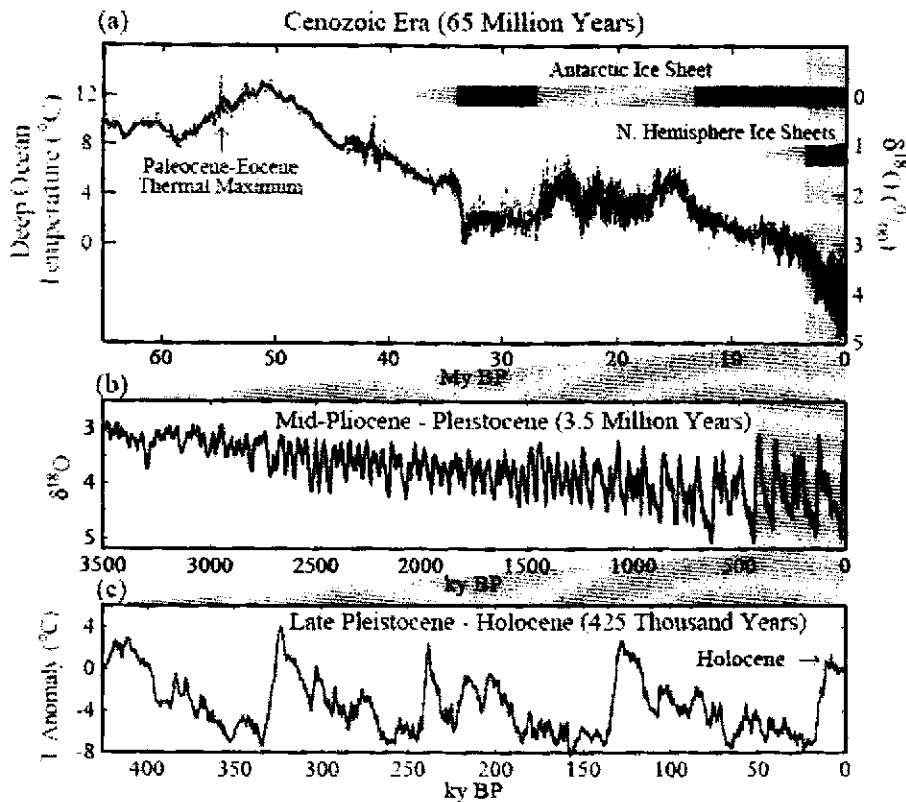
Figure 10. (a) Global compilation of deep-sea benthic foraminifera ^{18}\text{O} isotope records from Deep Sea Drilling Program and Ocean Drilling Program sites (Zachos et al 2001), temperatures applying only to ice-free conditions, thus to times earlier than \sim 35 My BP. The blue bar shows estimated times with ice present, dark blue being times when ice was equal or greater than at present. (b) Expansion of ^{18}\text{O} data for past 3.5 My. (Lisiecki and Raymo 2005) (c) Temperature data based on Vostok ice core (Vimeux et al 2002).
