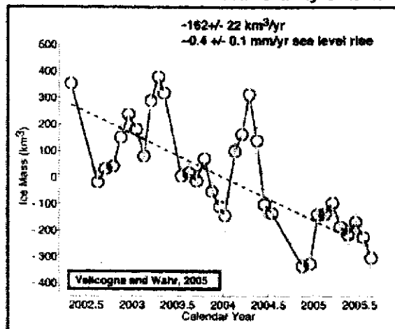
Figure 22. The GRACE satellite mission measures the Earth's gravitational field with such high precision that changes of the mass of the Greenland and Antarctic ice sheets can be measured. The ice sheet mass grows with winter snowfall and decreases during the melt season. Overall Greenland and West Antarctica are each now losing mass at rates of the order of 150 cubic kilometers of ice per year.
