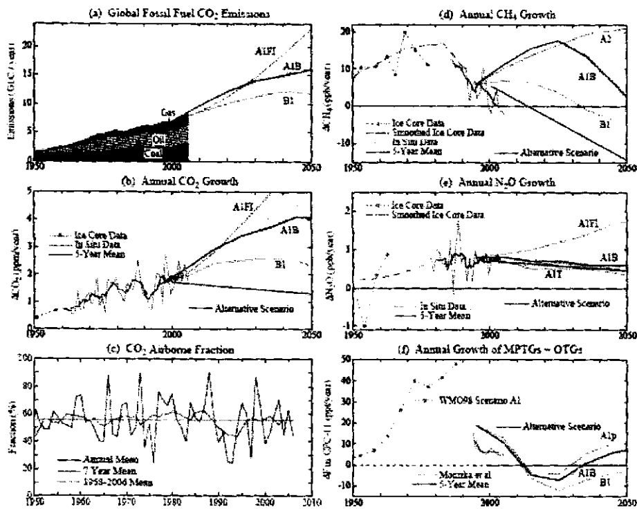
Figure 49. CO 2 emissions are increasing at a rate at or above IPCC “business-as-usual” scenarios. Other greenhouse gases are increasing at slower rates.
